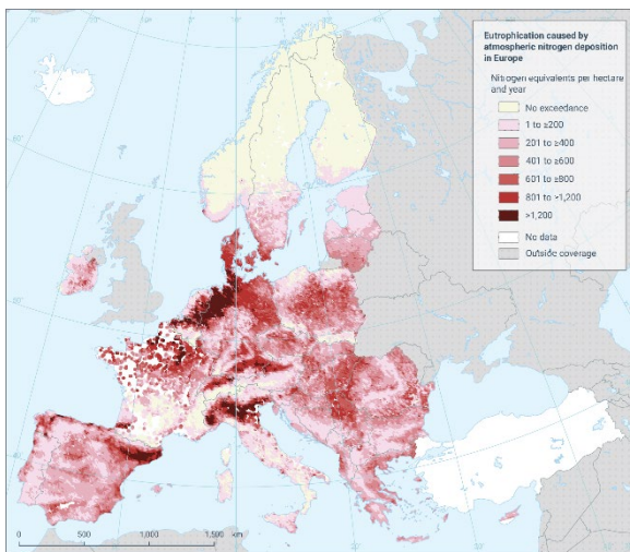
Exceedance of critical loads of atmospheric nitrogen deposition in Europe in 2021
