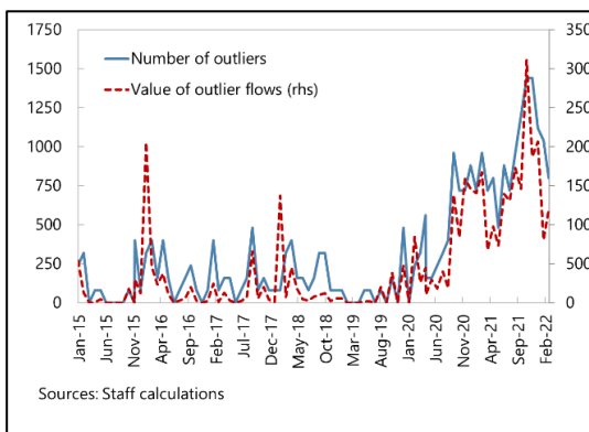
Figure 4. Outflows Outliers
