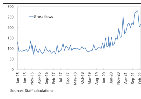
Figure 4. Outflows Outliers
