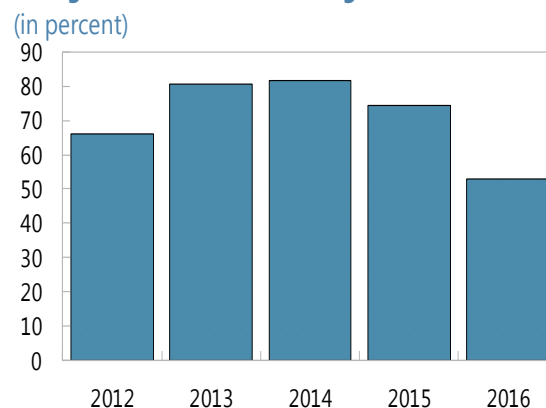
Foreign Reserves as a Percentage of the ARA Metric
