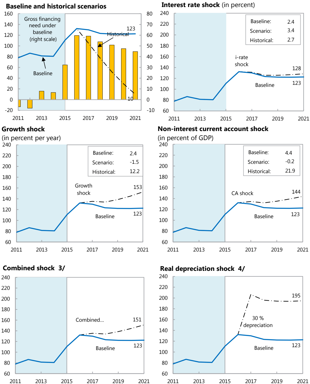
Figure 4. Qatar: External Debt Sustainability: Bound Tests 1/ 2/ (External debt in percent of GDP)
