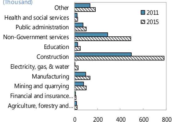
Workers in Paid Employment, 2011 and 2015
