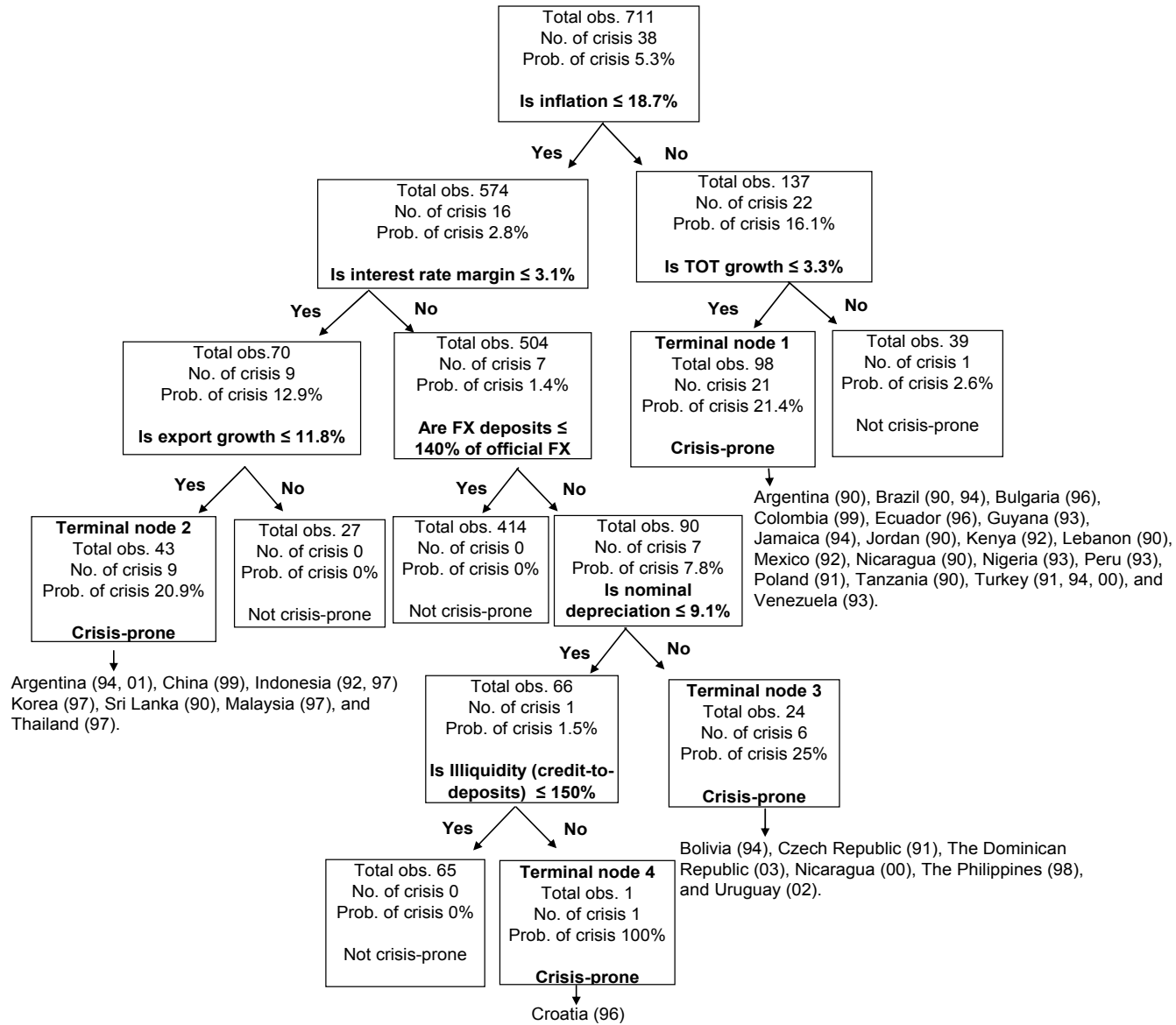
Figure IV.1. Binary Classification Tree, Baseline Model, 1990–2005
