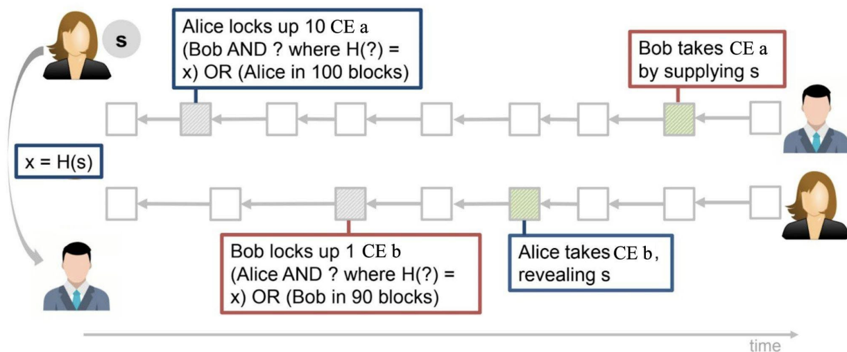
Figure 2.4. Hash Time Lock and Commitment, guaranteed instantaneous trade and settlement
