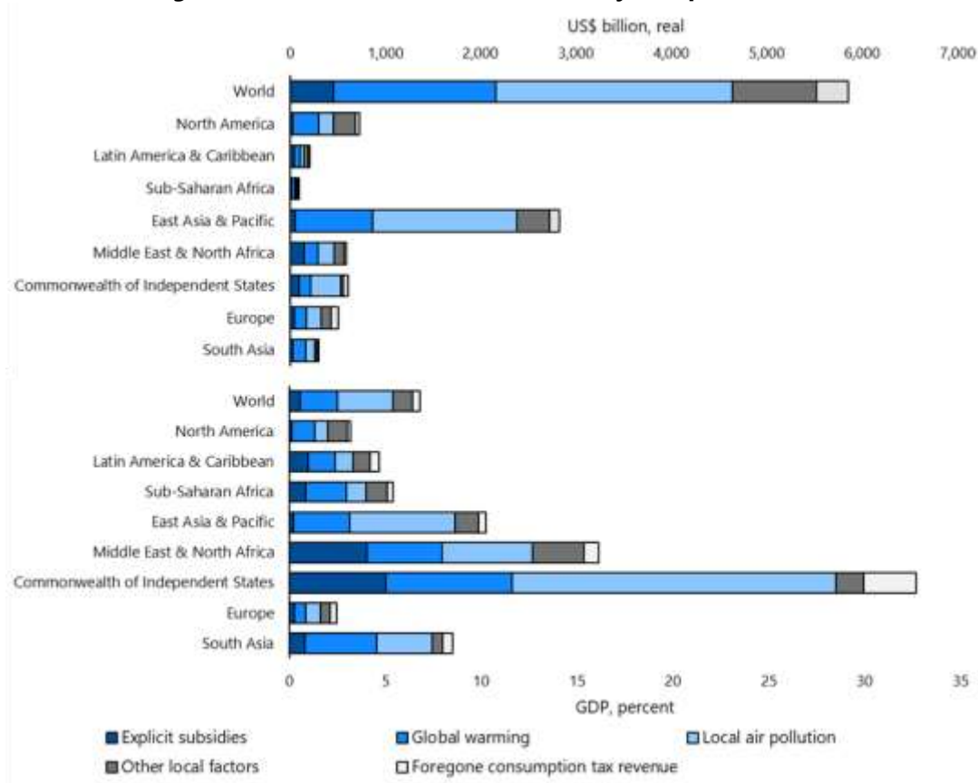
Figure ES3. Global Fossil Fuel Subsidies by Component, 2020
