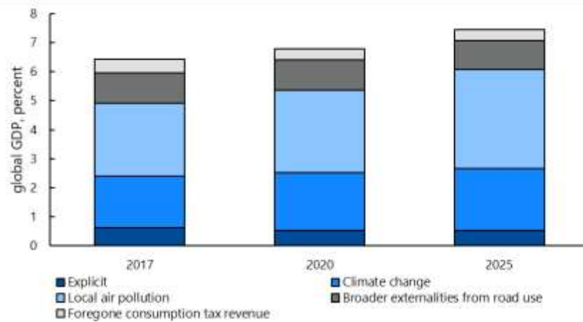
Figure 5. Global Fossil Fuel Subsidies by Component
