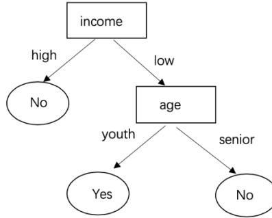
Figure B1. Decision Tree for Classifying Default
