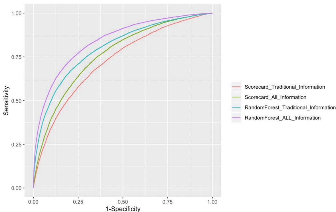
Figure 7: ROC Curves for Four Models
