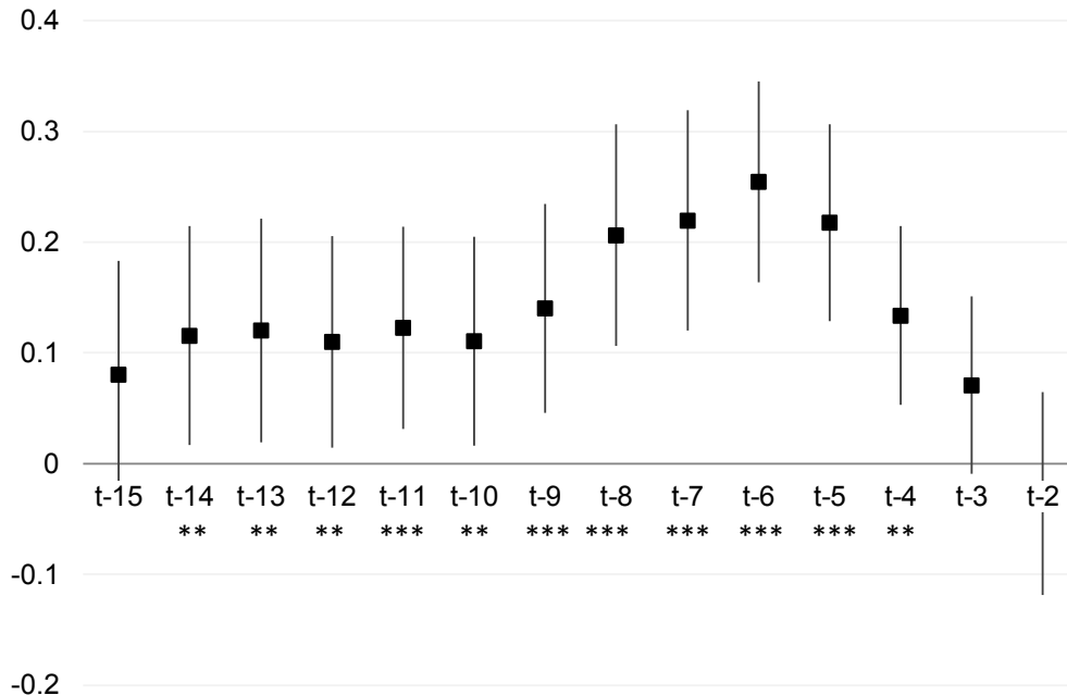
Figure 1: Estimates of \kappa in OLS regression (2) at the quarterly frequency when the dependent variable is real GDP growth, varying the lag \ell in \mu_{it-\ell} . Squares indicate the point estimate; lines capture the 95% confidence interval, calculated using cluster-robust standard errors. * denotes significance at the 10% level, ** implies significance at the 5% level, *** indicates significance at the 1% level.
