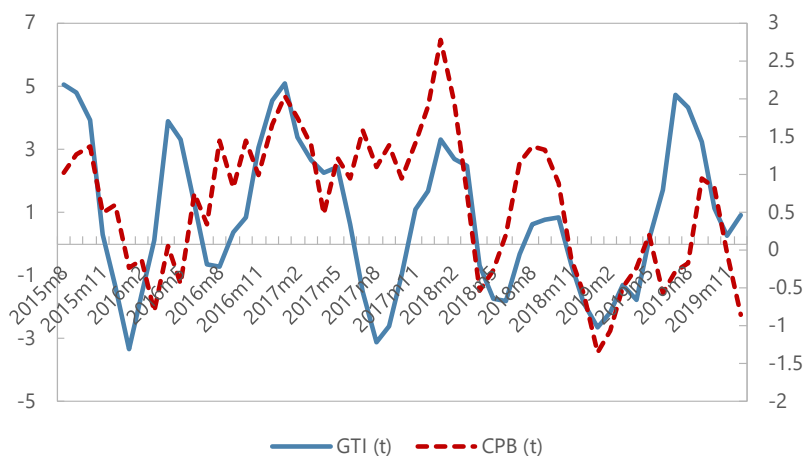
Figure 9. World: GTI Index and Official Data imports, 3m/3m growth rates, seasonally adjusted
