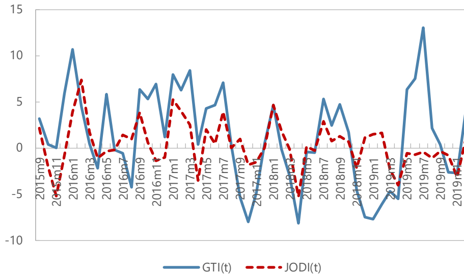
Figure 12. World: GTI and JODI crude oil import growth imports, 3m/3m growth rates, seasonally adjusted
