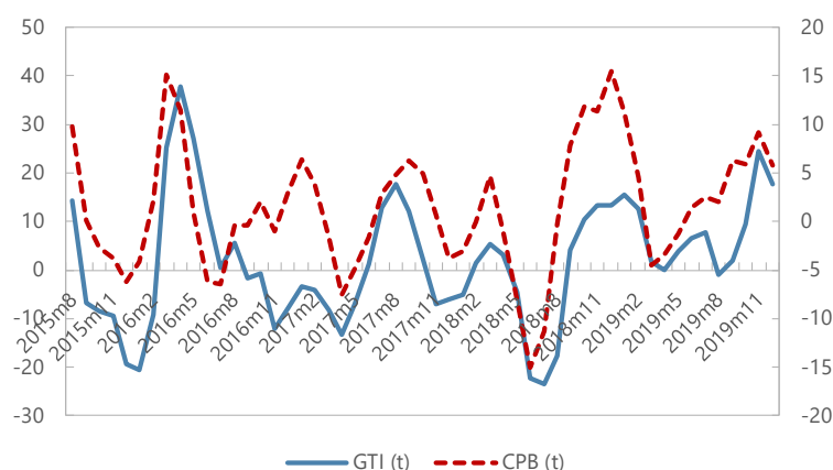
Figure 10. Argentina: GTI Index and Official Data exports, 3m/3m growth rates, seasonally adjusted
