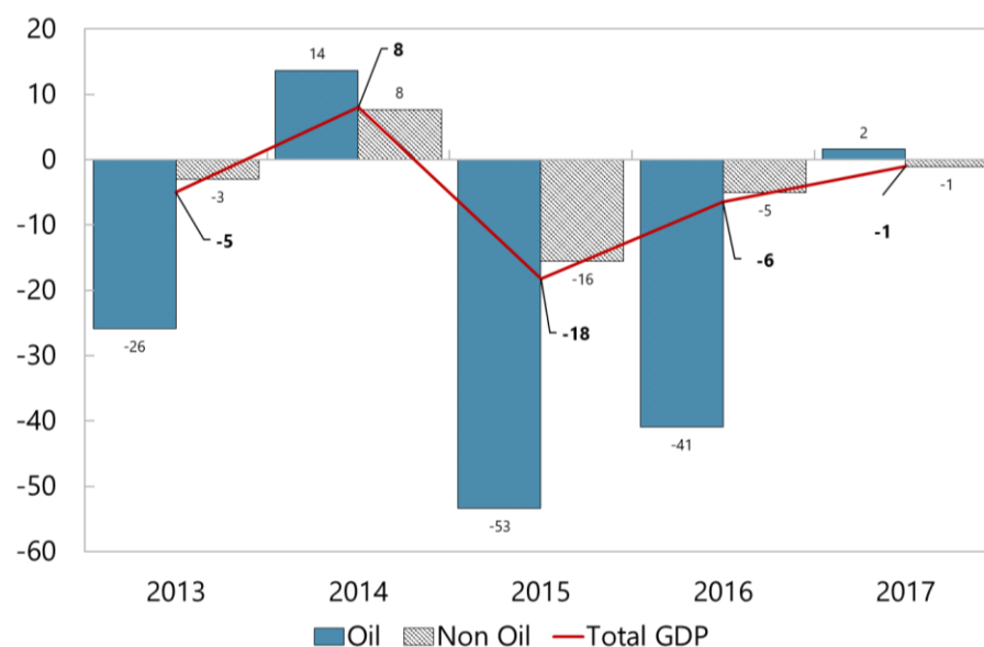
Figure 11. Decomposition of predicted real GDP growth in Yemen
