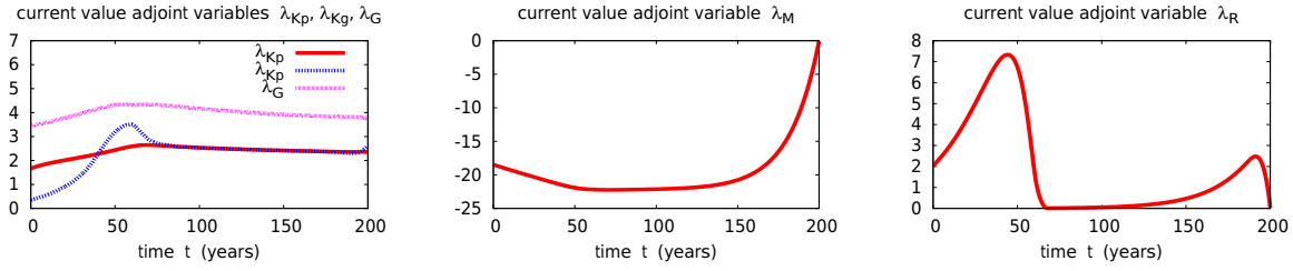
Figure 5: Adjoint variables for "small" initial values. (left) current value adjoint variables \lambda_{Kp}, \lambda_{Kg}, \lambda_G , (middle) current value adjoint variable \lambda_M , (right) current value adjoint variable \lambda_R .
