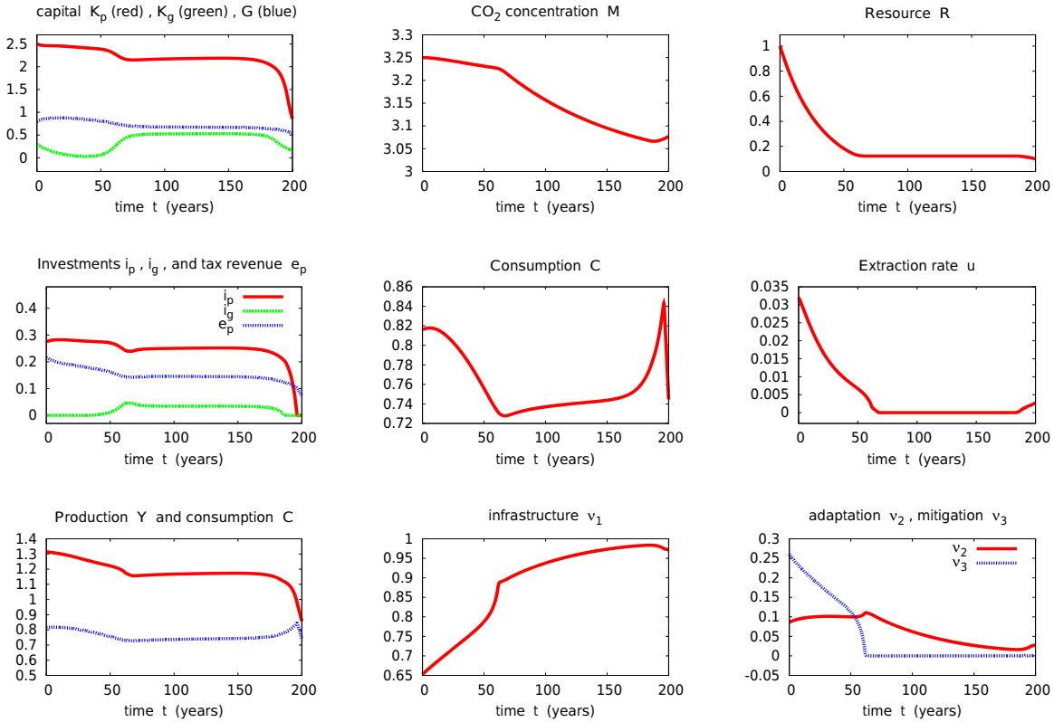
Figure 1: State and control trajectories for T = 200, K_p(0) = 2.5, K_g(0) = 0.3, G(0) = 0.8, M(0) = 3.25, R(0) = 1 , and free terminal state X(t_f) . Top row: (left) physical capital K_p , green capital K_g and government capital G , (middle) CO_2 concentration M , (right) resource R . Middle row: (left) investments i_p, i_g and tax revenue e_p , (middle) consumption C (right) extraction rate u . Bottom row: (left) consumption C and productivity Y , (middle) infrastructure \nu_1 , (right) adaptation \nu_2 and mitigation \nu_3 .
