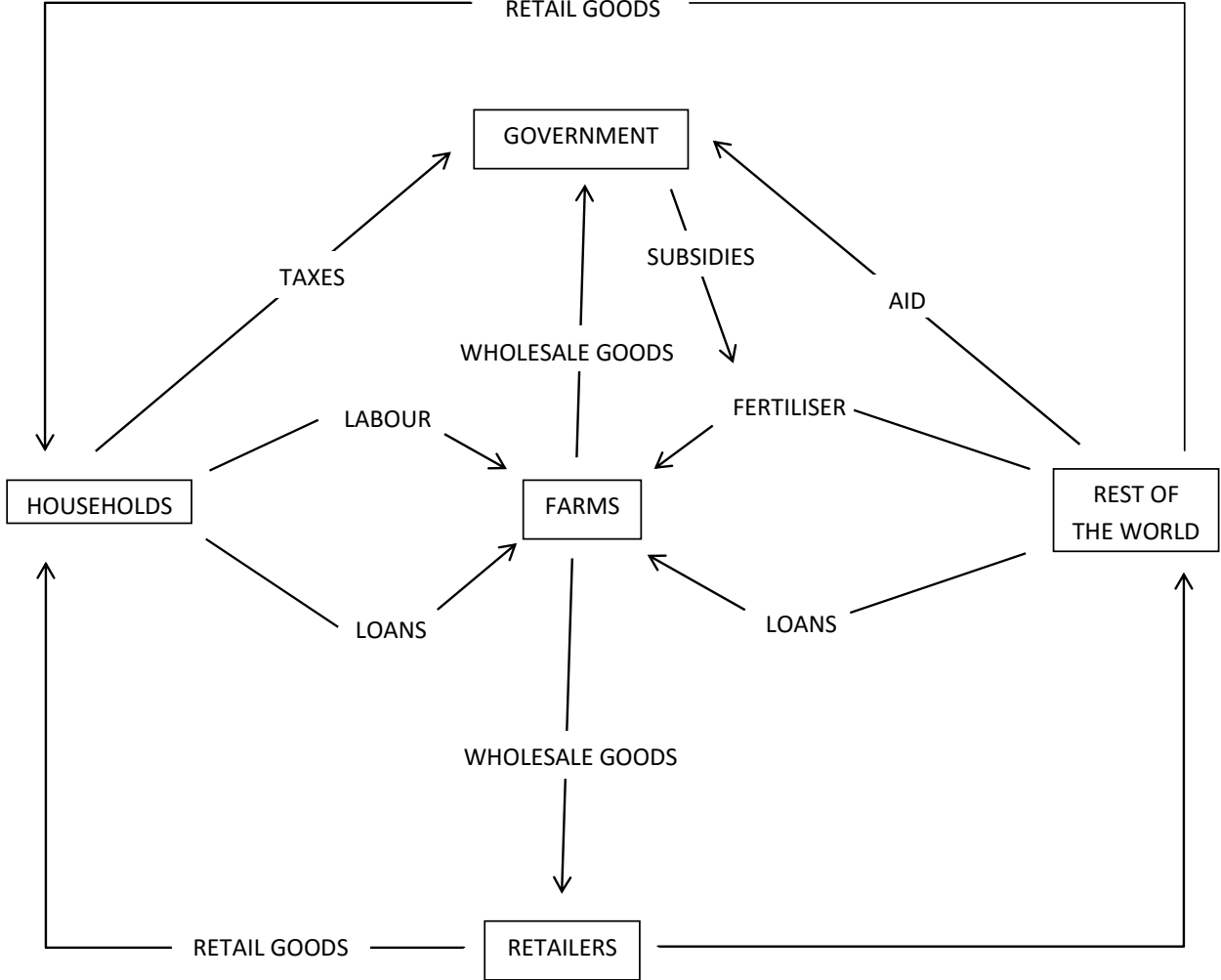
Figure 1. Model overview
