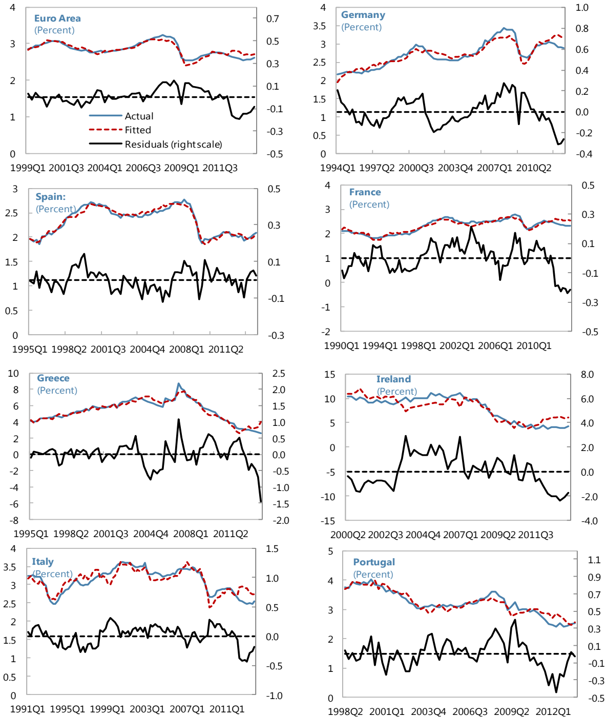
Figure 1. A2. Leaked Model: Private Non-residential Investment/Capital Ratio
