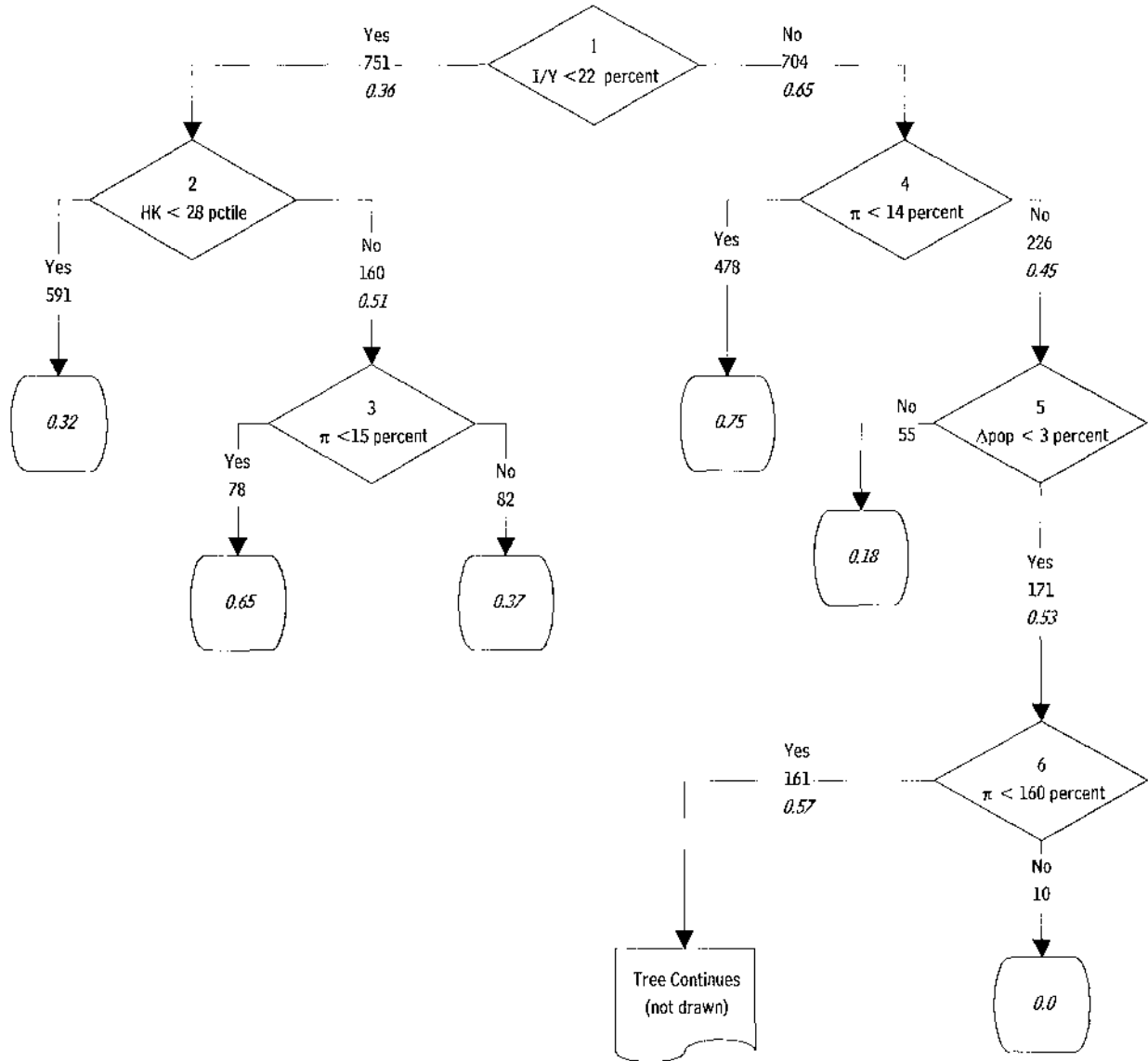
Figure 6: Binary Recursive Tree of High vs. Low GDP Growth
