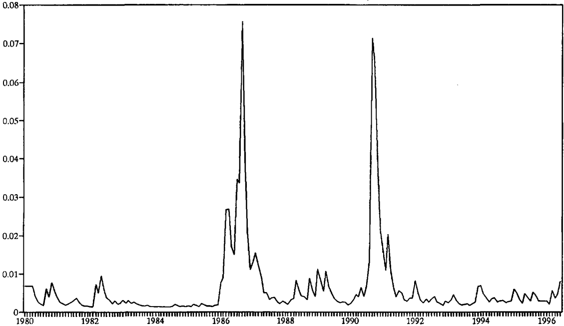
Figure 2. Estimated Conditional Variance of Oil Prices, Jan 1980-Jun 1996.
