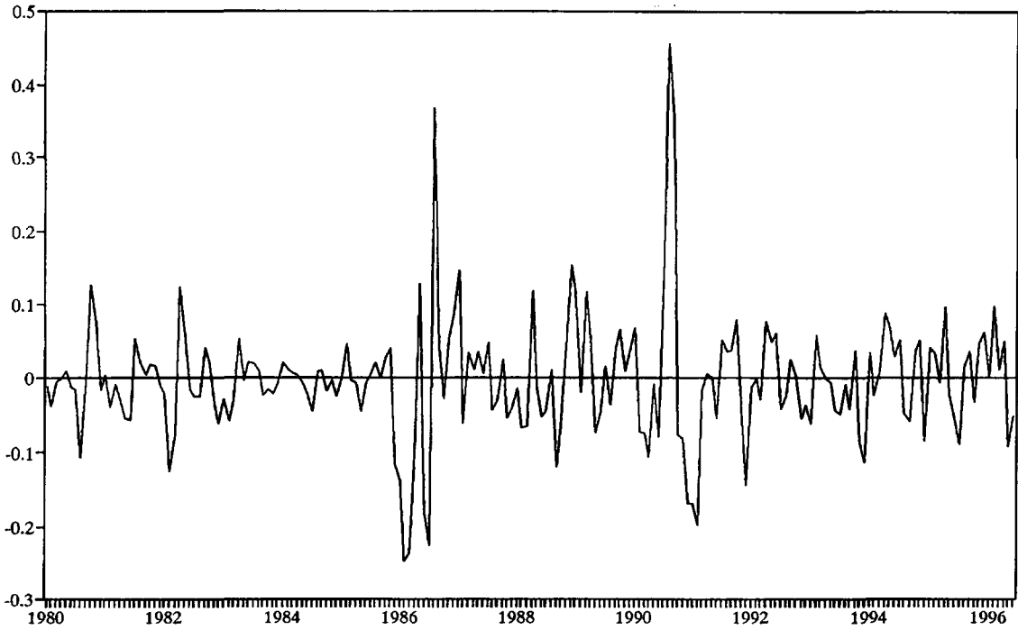
Figure 1. First Difference of the Log of monthly Crude Oil prices, Jan 1980-Jun 1996. 1/
