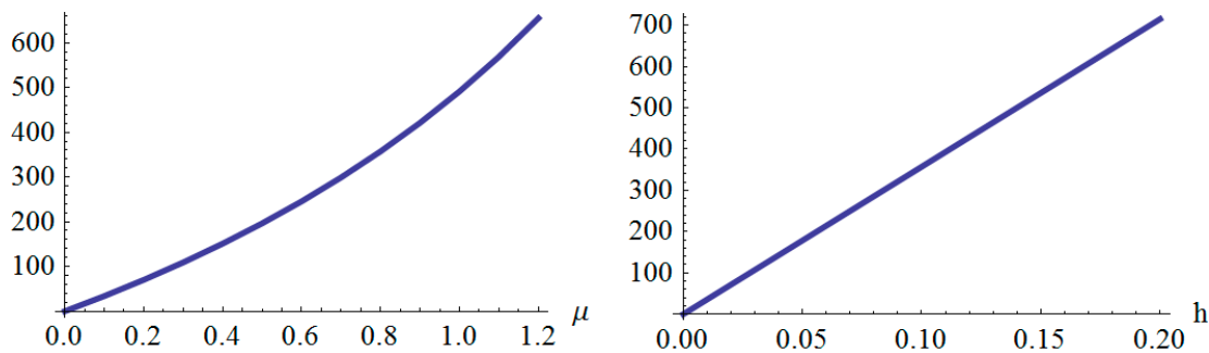
Figure 2: Interest rate threshold with constant multipliers and no natural closing of the output gap until Time 4 (basis points above 1/\beta )
